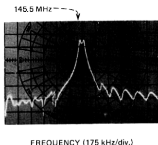
Fig. 10—(a) Diagram of a multistrip-coupled resonator-filter pair. (b) The electrical transmission spectrum in a 50 \Omega system for a multistrip ( 5 \mu\text{m} strips, L_5 = 90 \mu\text{m} ) coupled resonator-filter-pair on YZ-LiNbO 3 with L_1 = L_6 = 9.60 \text{ mm} , \Delta = 12 \mu\text{m} , N_t = 5 and an acoustic aperture in each track of 50 wavelengths. (c) The calculated transmission spectrum of the device in (b) with q = 0.163 , \kappa = 4.3 \text{ cm}^{-1} , \alpha/\kappa = 0.01 , R_s = 10 \Omega , \epsilon_m = 0.047 , \phi_2 = 0.25 \pi and \phi_4 = 9.89 \pi on resonance.
