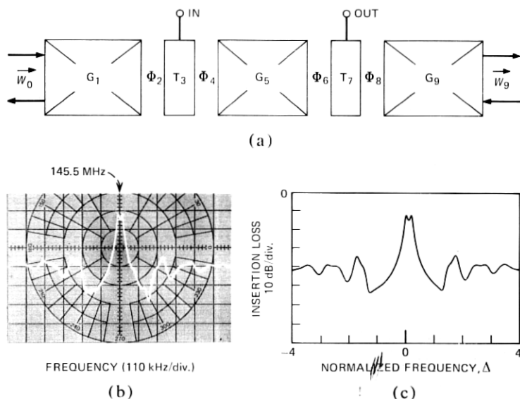
Fig. 9—(a) Diagram of an acoustically cascaded resonator-filter pair. (b) The electrical transmission spectrum in a 50\ \Omega system for an acoustically cascaded resonator-filter pair on YZ-LiNbO 3 with L_1 = L_9 = 9.60 mm, L_5 = 7.296 mm, \Lambda = 12\ \mu\text{m} , N_t = 5 and an acoustic aperture of 50 wavelengths. (c) The calculated spectrum for the device in (b) using \kappa = 3.3\ \text{cm}^{-1} , \alpha/\kappa = 0.01 , R_s = 12\ \Omega , \epsilon_g = 0.018 and \phi_2 = \phi_4 = \phi_6 = \phi_8 = 0.234\ \pi on resonance.
