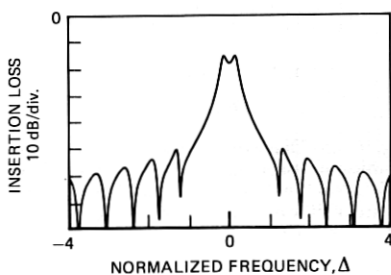
Fig. 10—(a) Diagram of a multistrip-coupled resonator-filter pair. (b) The electrical transmission spectrum in a 50 \Omega system for a multistrip ( 5 \mu\text{m} strips, L_5 = 90 \mu\text{m} ) coupled resonator-filter-pair on YZ-LiNbO 3 with L_1 = L_6 = 9.60 \text{ mm} , \Delta = 12 \mu\text{m} , N_t = 5 and an acoustic aperture in each track of 50 wavelengths. (c) The calculated transmission spectrum of the device in (b) with q = 0.163 , \kappa = 4.3 \text{ cm}^{-1} , \alpha/\kappa = 0.01 , R_s = 10 \Omega , \epsilon_m = 0.047 , \phi_2 = 0.25 \pi and \phi_4 = 9.89 \pi on resonance.
